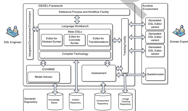
Figure 5: Architecture Overview
